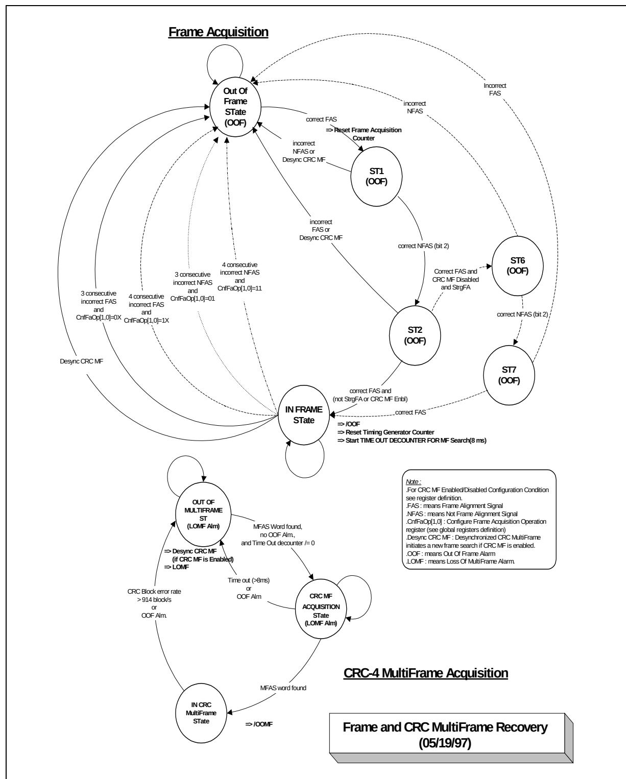
Figure 5. Frame and Multiframe Acquisition
