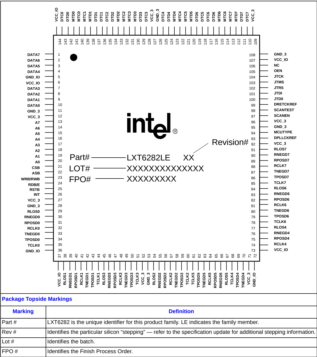
Figure 4. LXT6282 Pin Assignment
