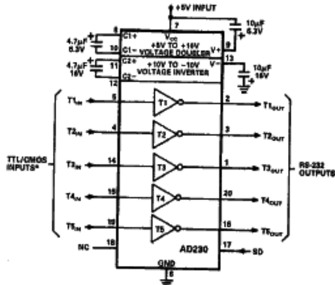
*INTERNAL 600kΩ PULL-UP RESISTOR ON EACH TTL/CMOS INPUT Figure 2. AD230 Typical Operating Circuit
