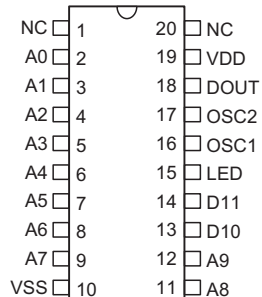
HT6012 -20 SOP-A
