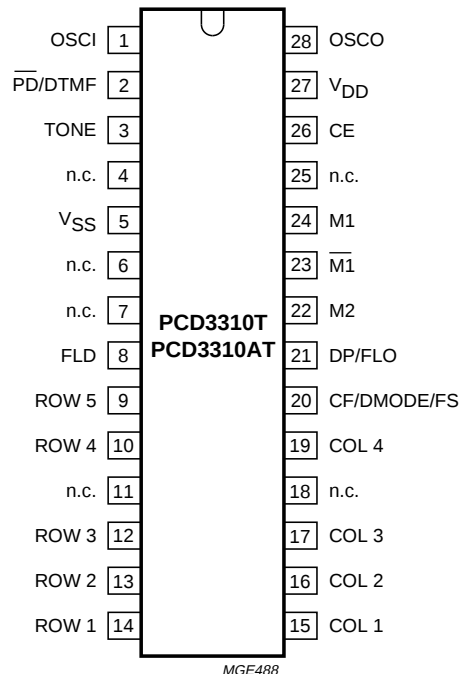
Fig.3 Pin configuration (SO28 package).
