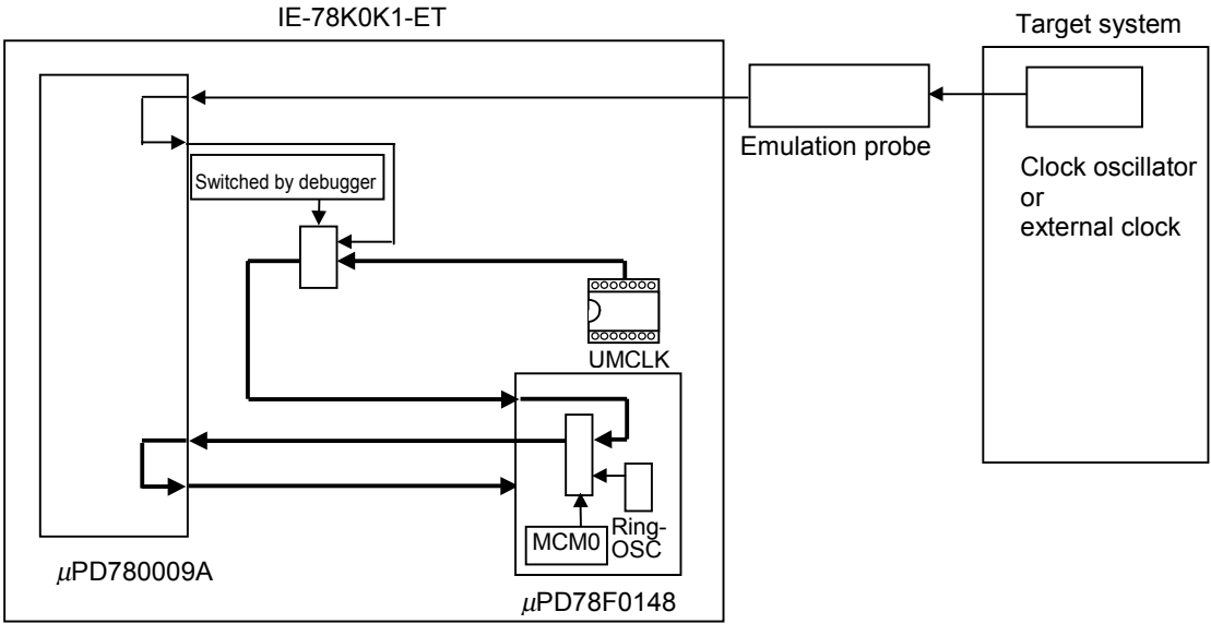
Figure 3-8. Flow of Clock (Main System Clock)
