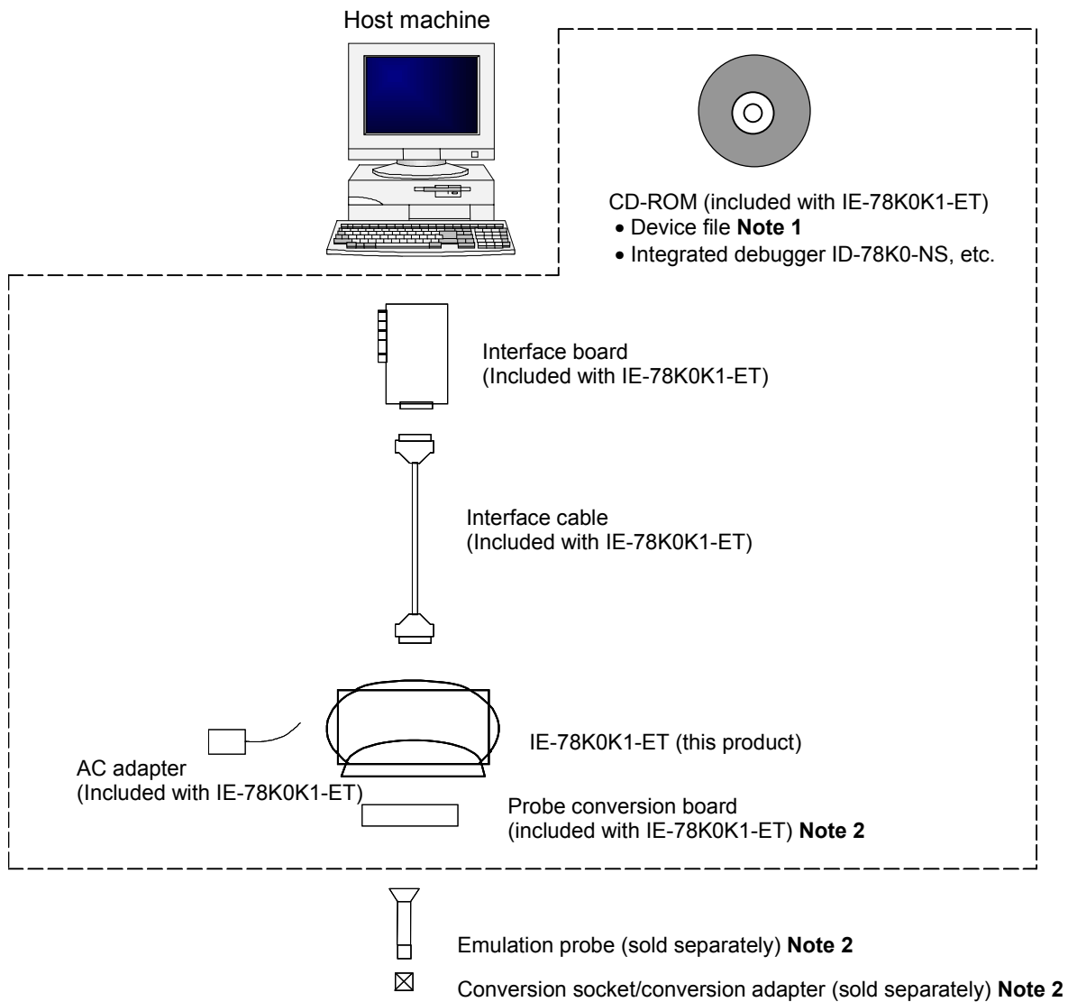
Figure 1-1. System Configuration
