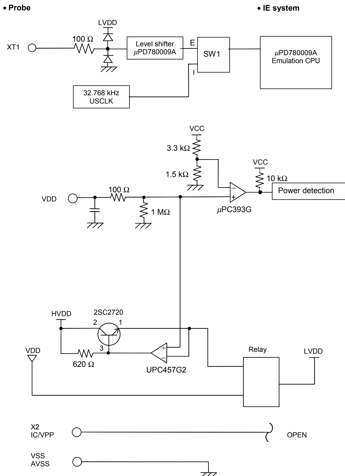
Figure 4-3. Equivalent Circuit of Emulation Circuit (c)
