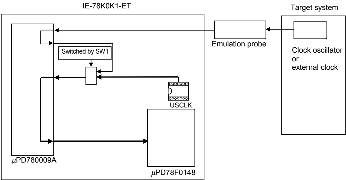
Figure 3-9. Flow of Clock (Subsystem Clock)
