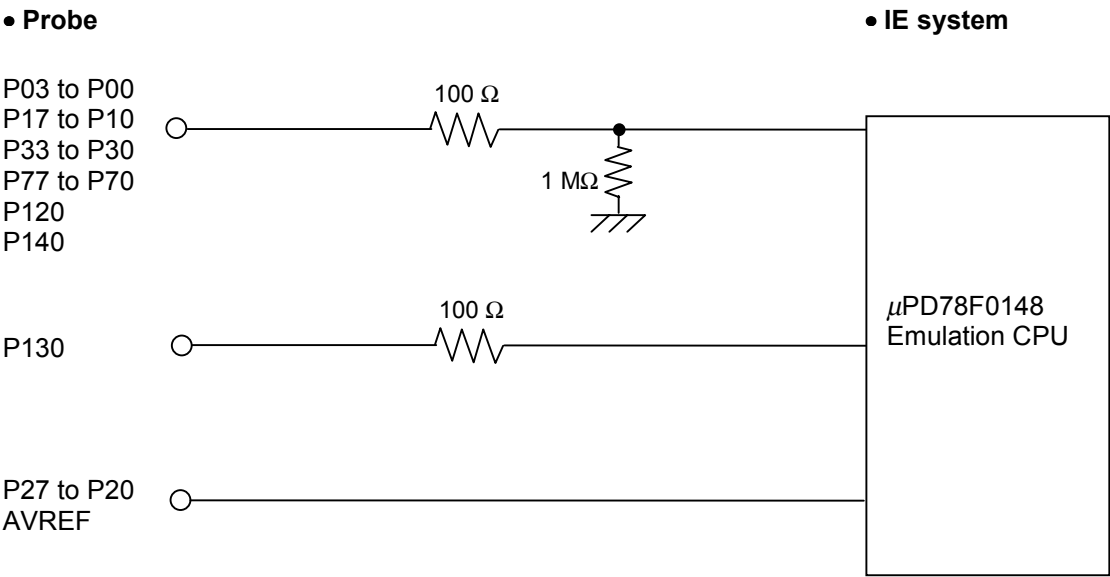
Figure 4-9. Equivalent Circuit of Emulation Circuit (b)
