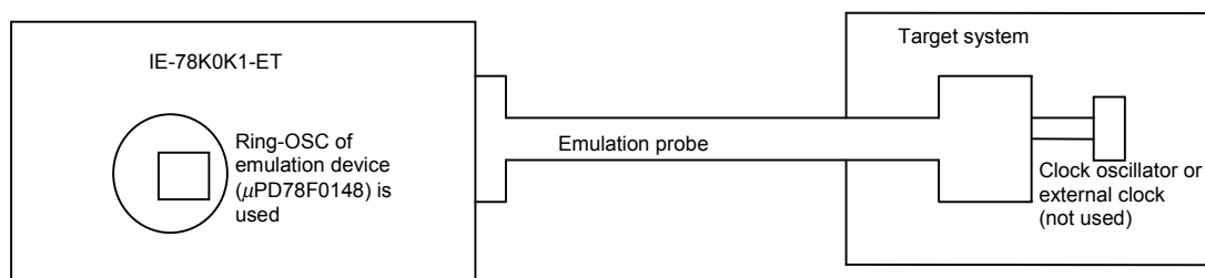
Figure 3-19. When Using Ring-OSC (Main System Clock)
