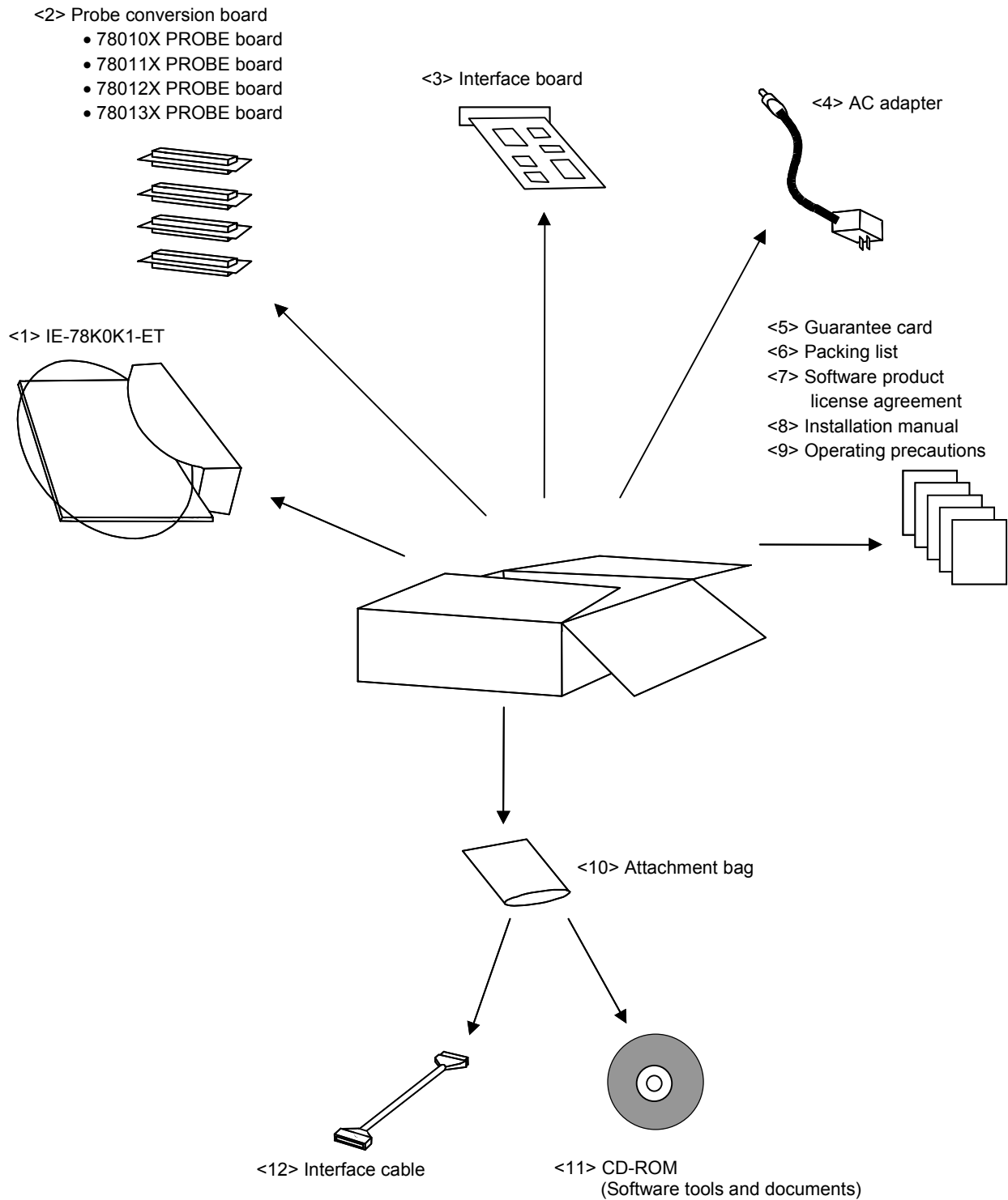
Figure 1-3. Package Contents
