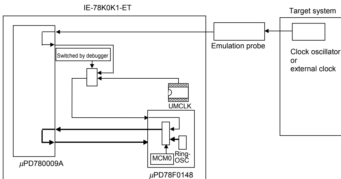
Figure 3-20. Flow of Clock (Main System Clock)
