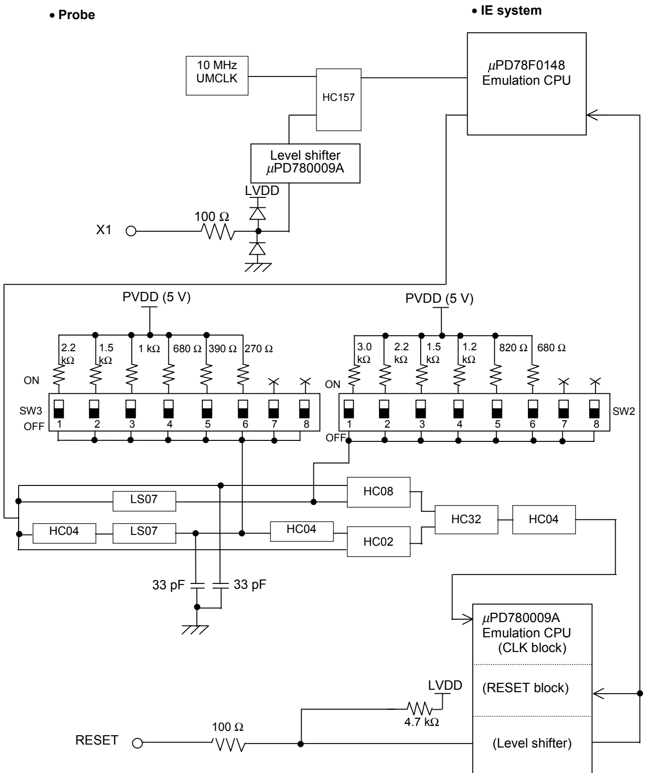
Figure 4-10. Equivalent Circuit of Emulation Circuit (c)
