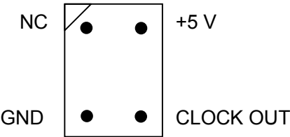
Figure 3-13. Crystal Oscillator (Main System Clock)
