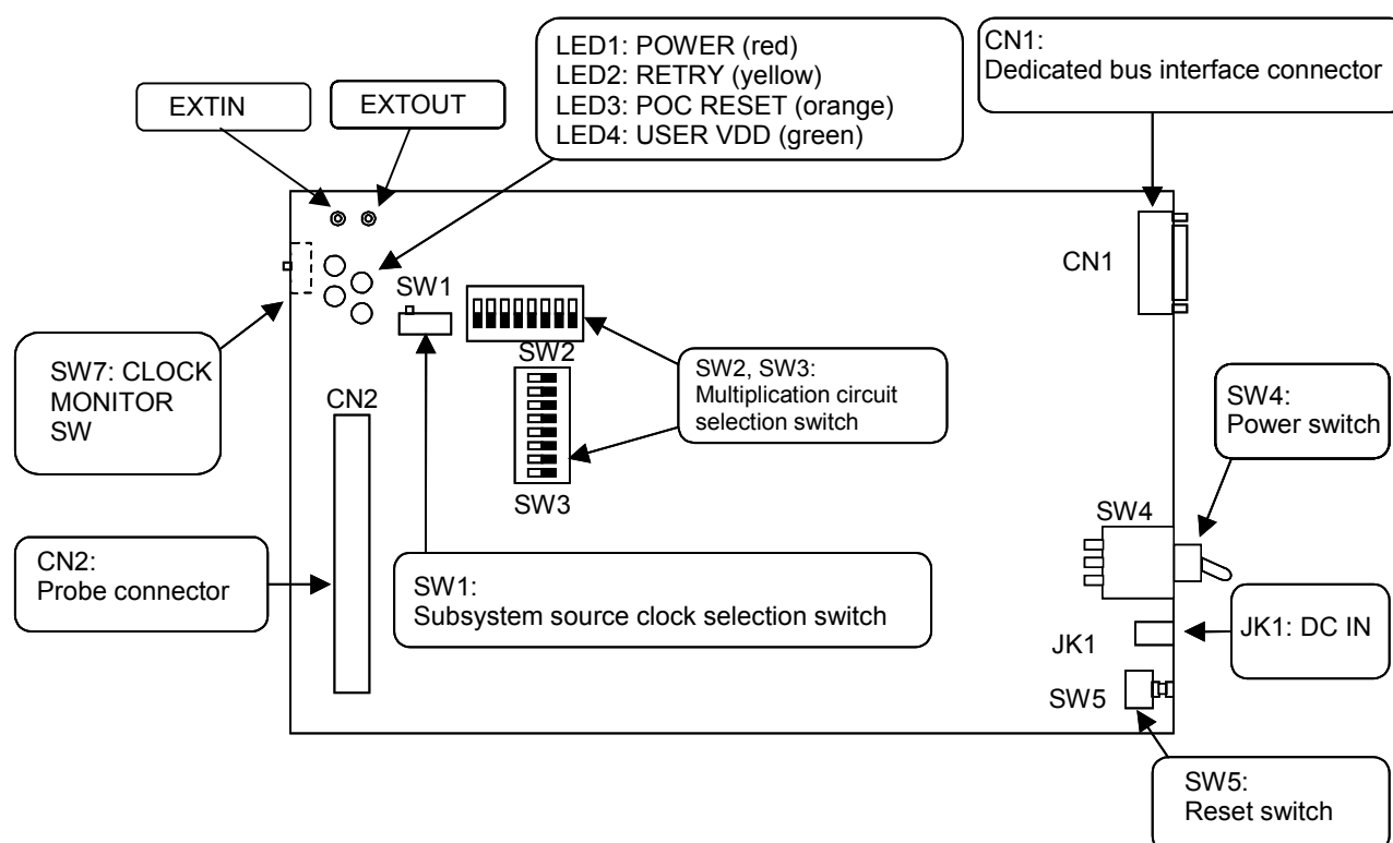
Figure 3-21. Package Drawing of Emulation board (S-780148 Board)
