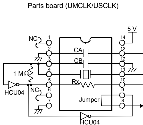
Figure 3-15. Connections on Parts Board
