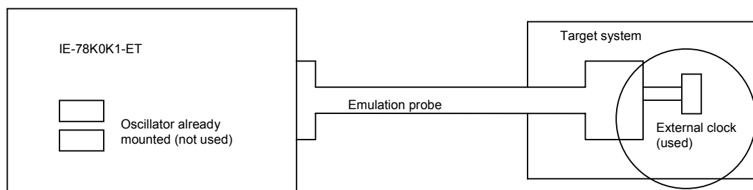
Figure 3-16. When Using Clock Input from Target System (Main System Clock)
