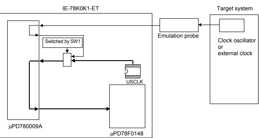
Figure 3-12. Flow of Clock (Subsystem Clock)
