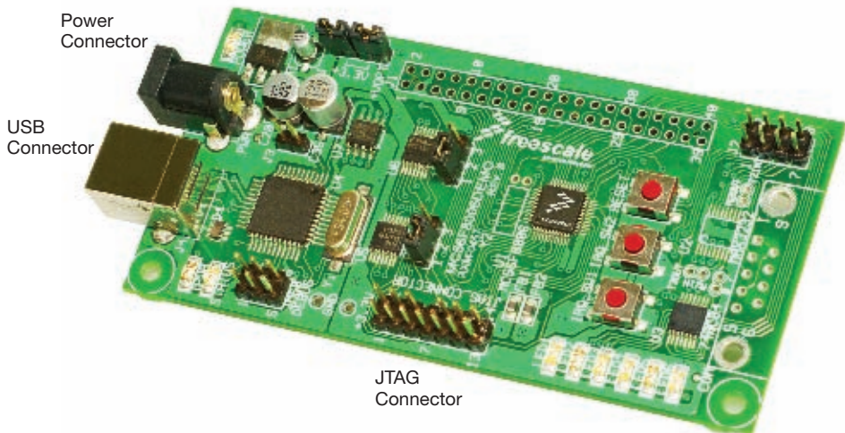
Figure 1. MC56F8006DEMO-T
