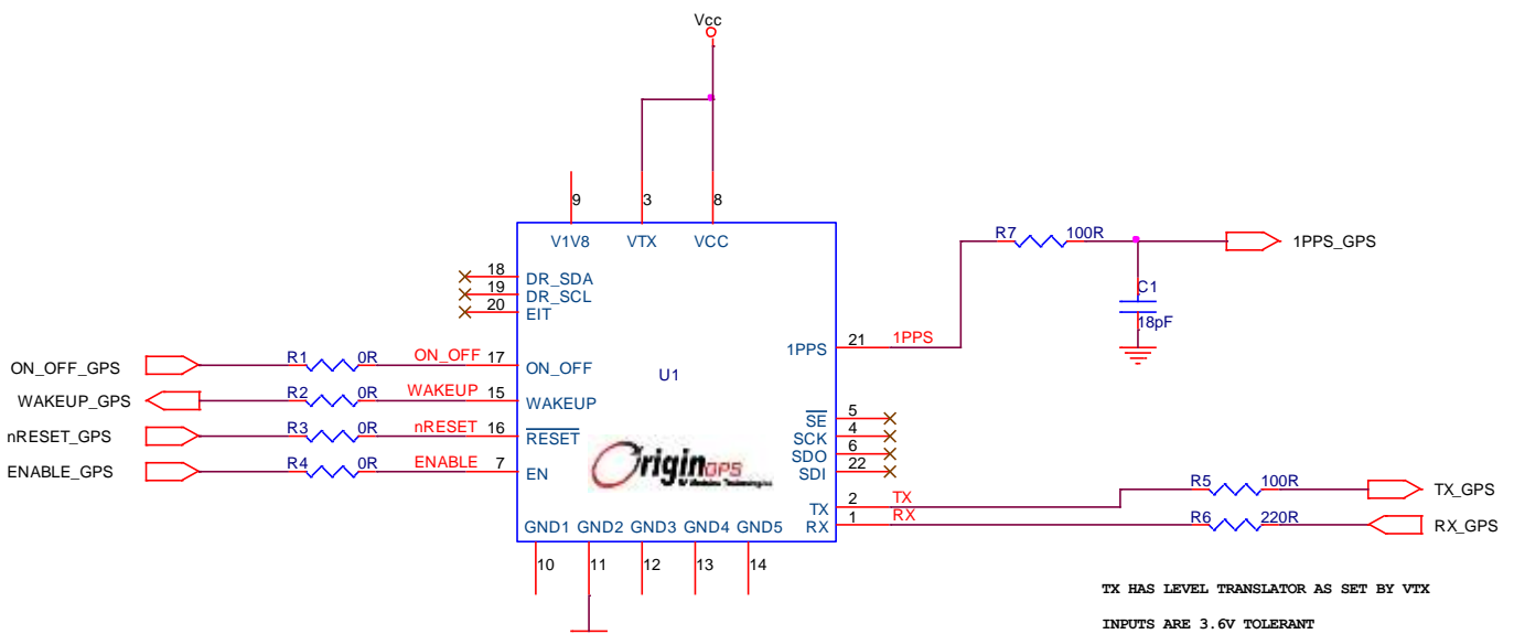
FIGURE 10 – UART INTERFACE CIRCUIT
