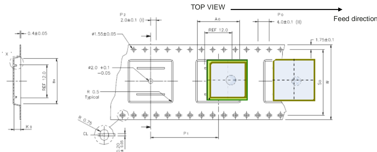
FIGURE 16 – CARRIER
