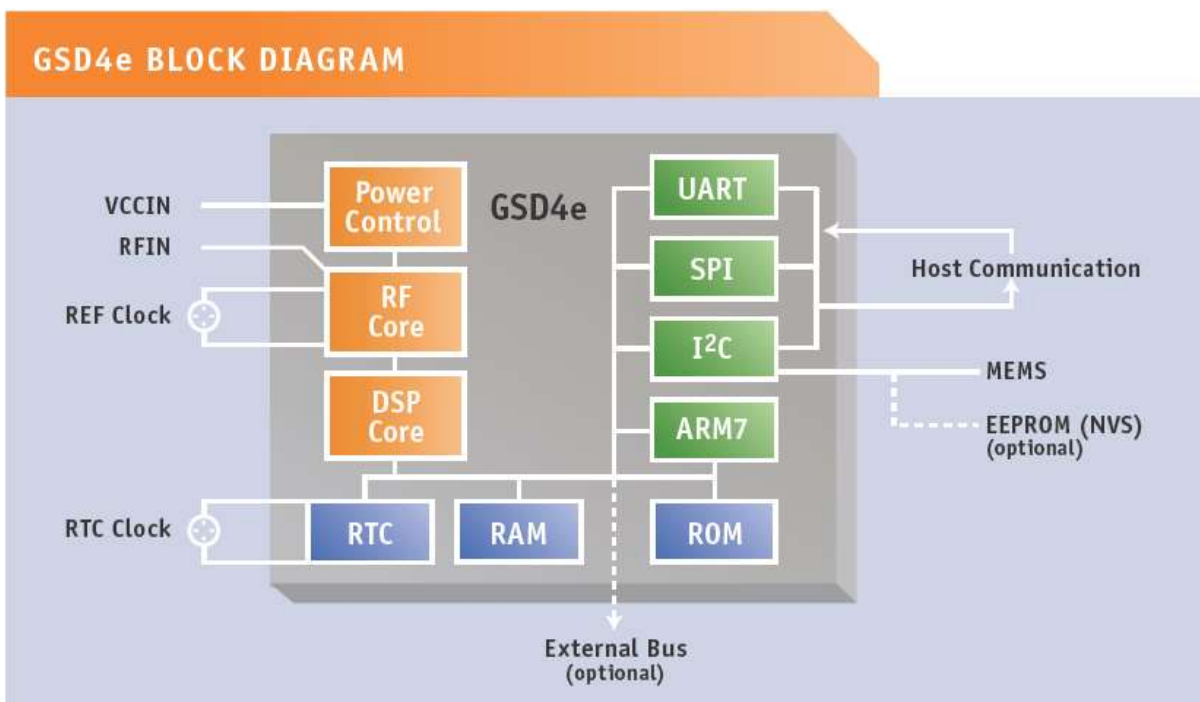
FIGURE 2 – GSD4e FUNCTIONAL BLOCK DIAGRAM
