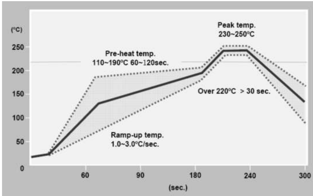
FIGURE 18 – RECOMMENDED SOLDERING PROFILE
