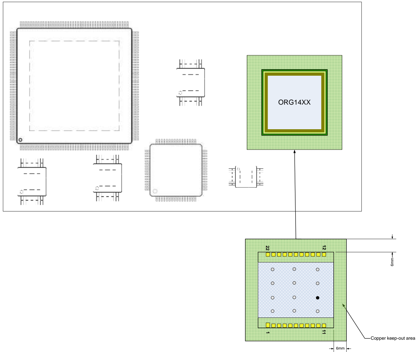
FIGURE 13 – ORG14XX MODULE PLACEMENT
