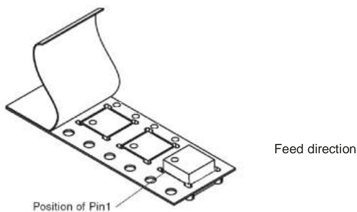
FIGURE 17 – MODULE POSITION
