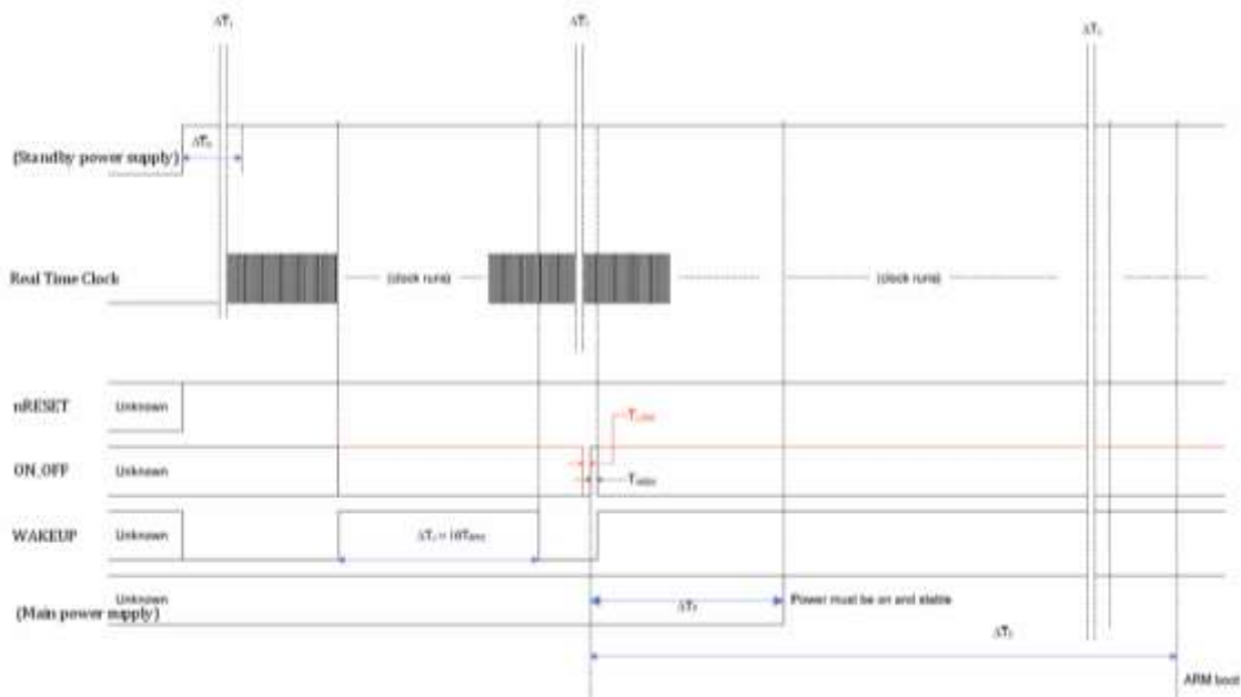
FIGURE 15 – STARTUP TIMING
