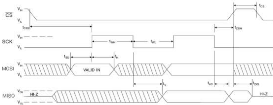
FIGURE 9 – SPI TIMING
