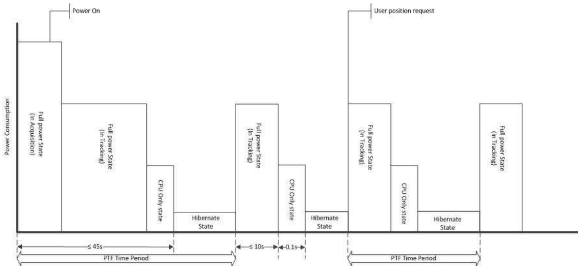
FIGURE 4 – PTF™ TIMING
