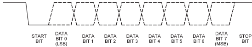
FIGURE 8 – UART INTEGRITY
