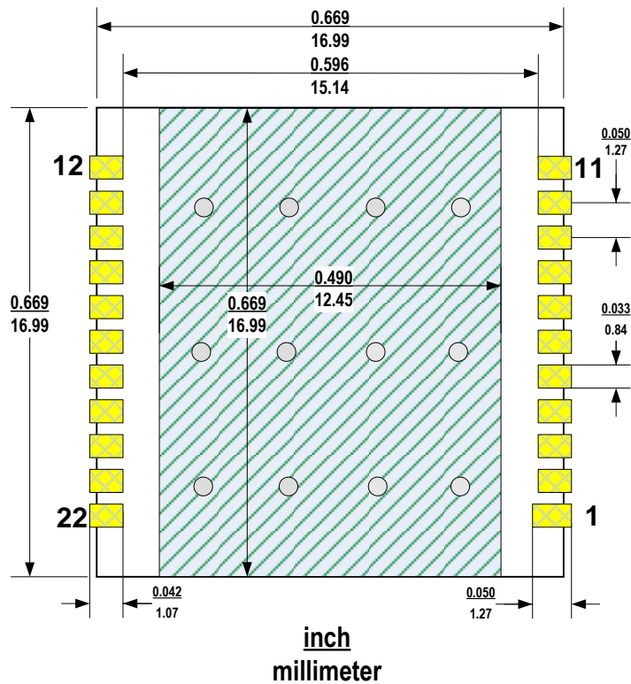
FIGURE 12 – FOOTPRINT
