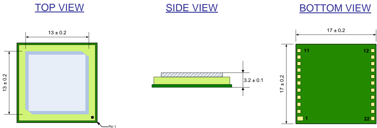
FIGURE 19 – ORG1400 MECHANICAL DRAWING
