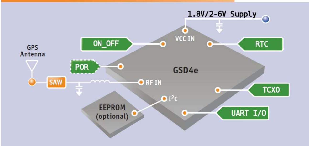
FIGURE 1 – ORG14XX ARCHITECTURE
