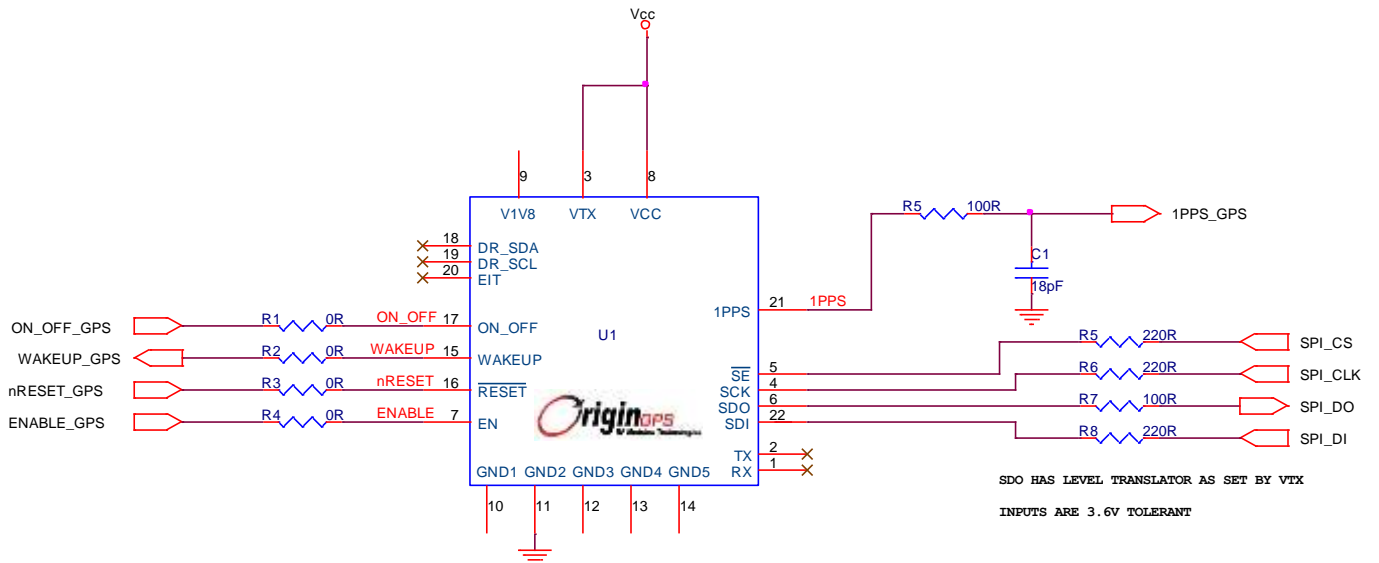
FIGURE 11 – SPI INTERFACE CIRCUIT
