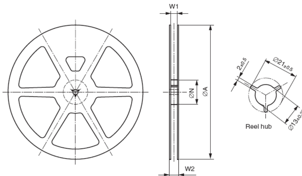
Figure 10-3: Reel
