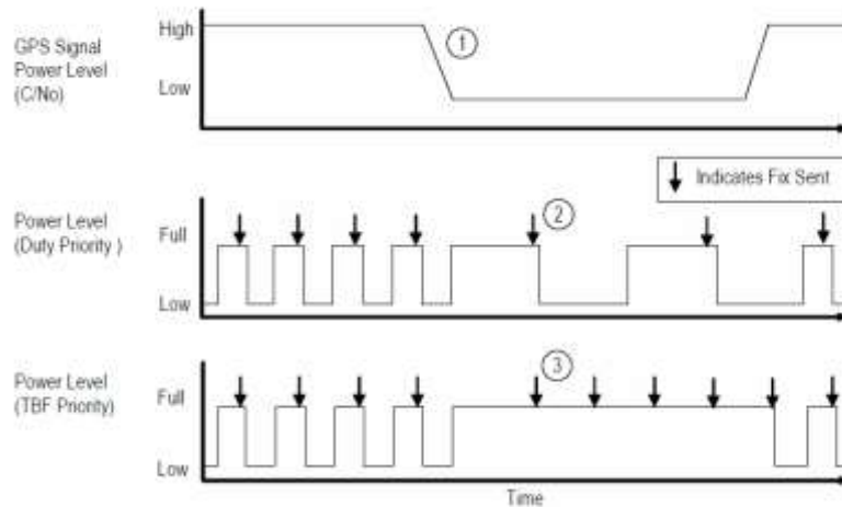
FIGURE 5 – APM™ TIMING
