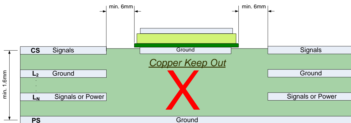
FIGURE 14 – TYPICAL PCB STACK UP
