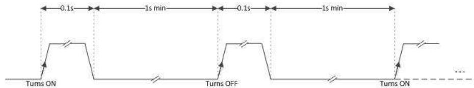
FIGURE 7 – RECOMMEND ON_OFF TIMING
