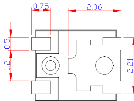
< Figure 1 PLCC 3528 series Dimensions >
