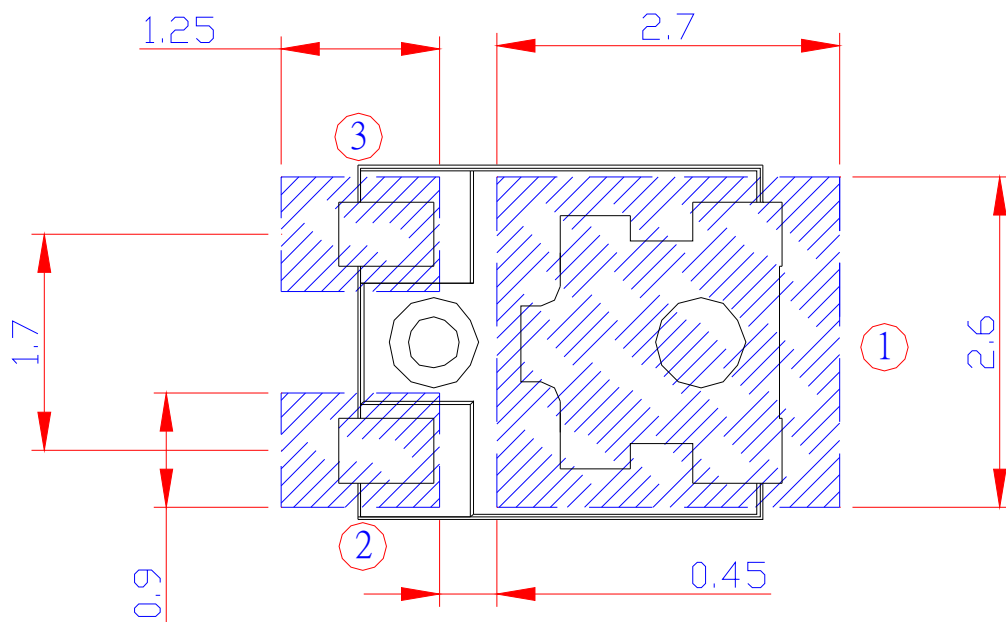
<Figure 8.Pad Dimension >
