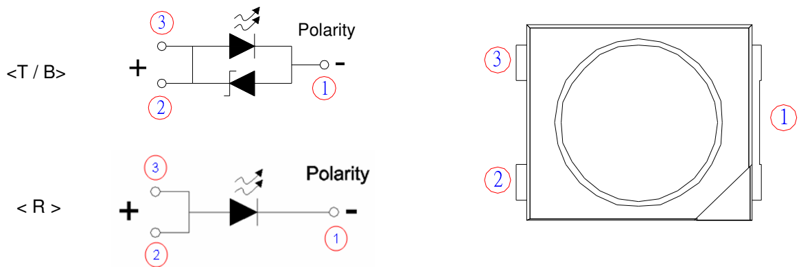
< Figure 2 PLCC 3528 series circuit diagram >
