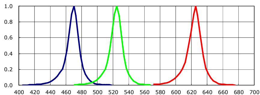
< Figure 4 Wavelength & relative intensity for PLCC 3528 series.>
