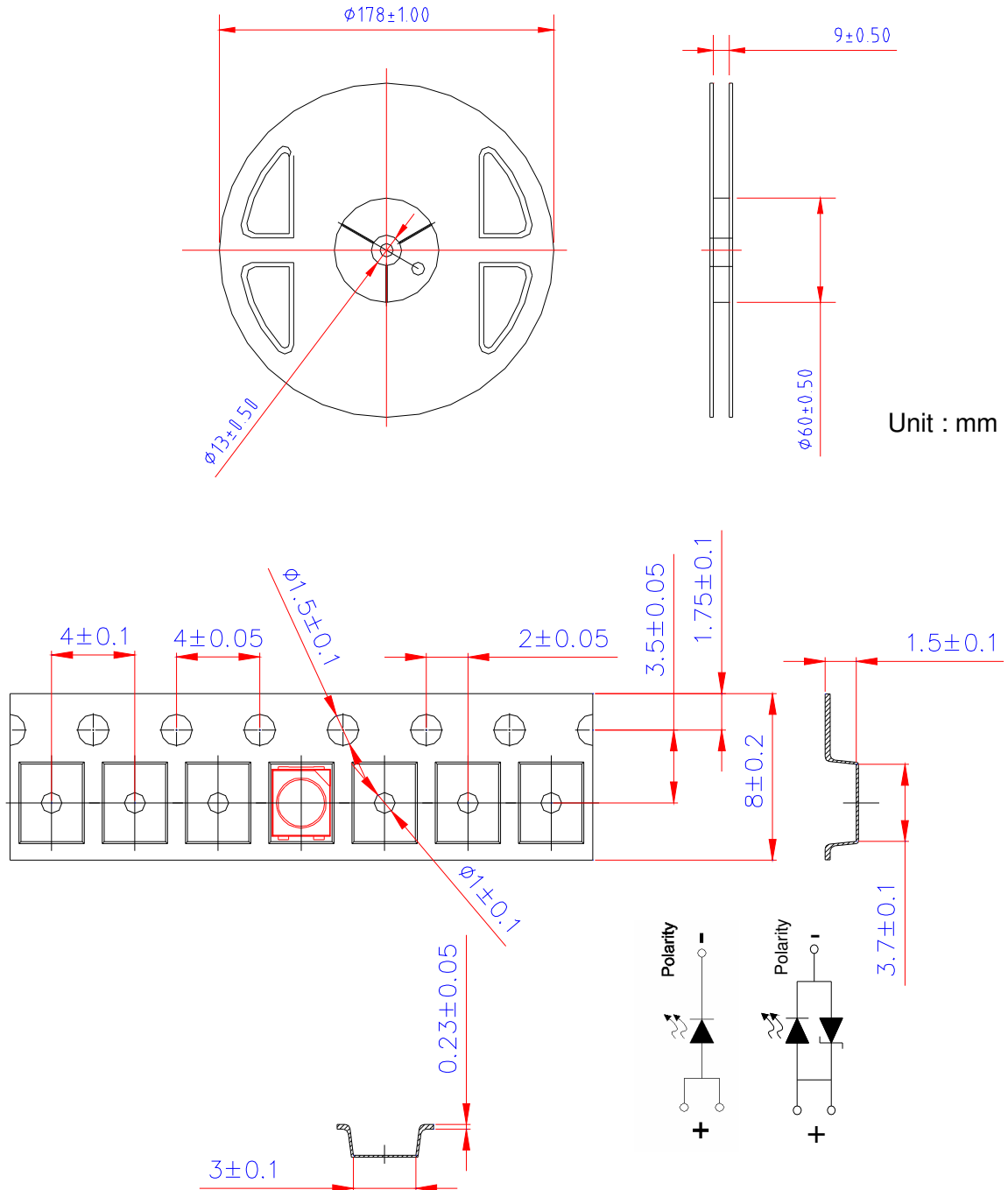
< Figure 10 Taping reel dimensions >
