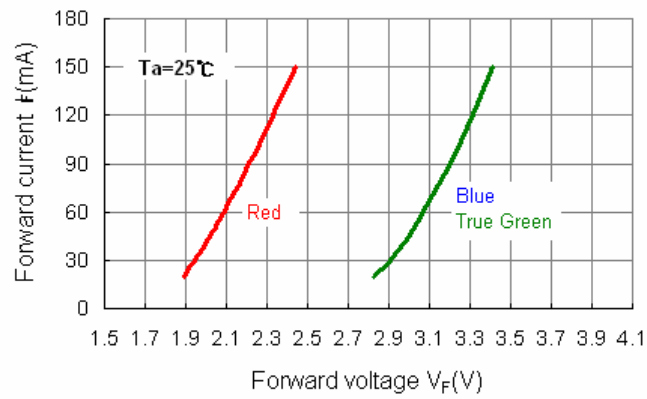
< Figure 6 Forward voltage & forward current for PLCC 3528 series >
