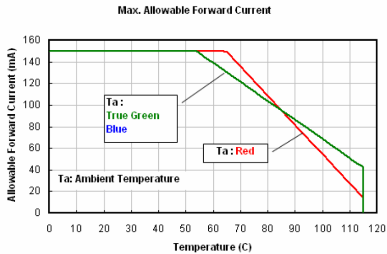
< Figure 7 Ambient temperature & forward current for PLCC 3528 series >
