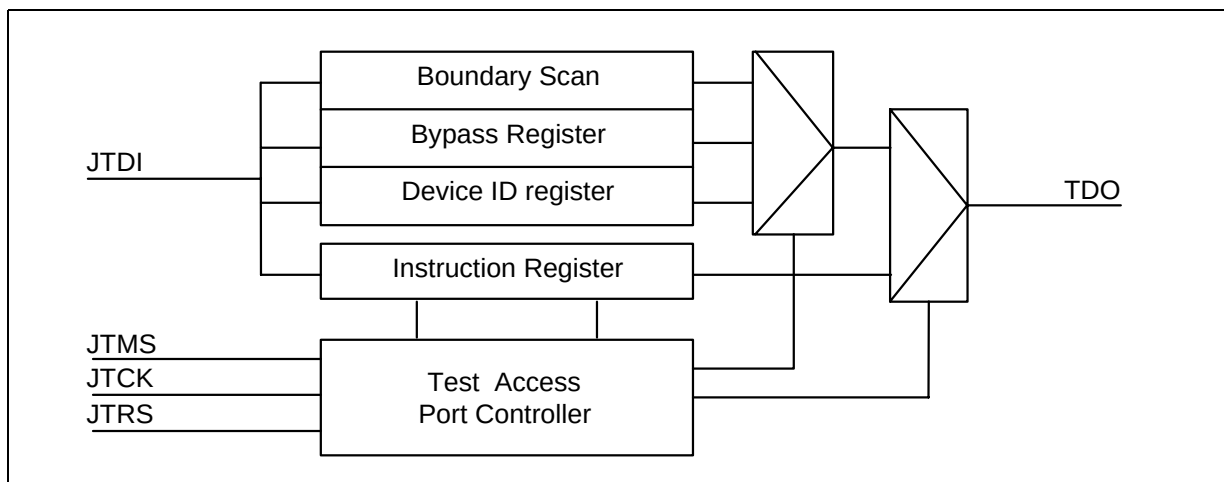
Figure 49. Test Access Port
