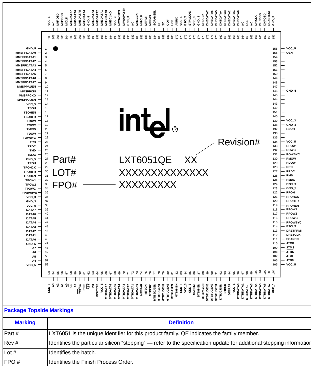
Figure 2. LXT6051 Pin Assignment
