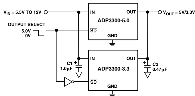
Figure 22. Crossover Switch
