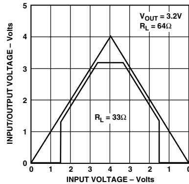
Figure 9. Power-Up/Power-Down
