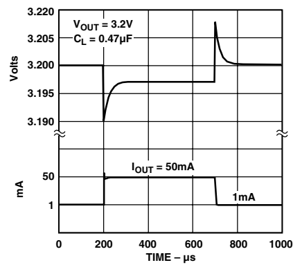
Figure 13. Load Transient
