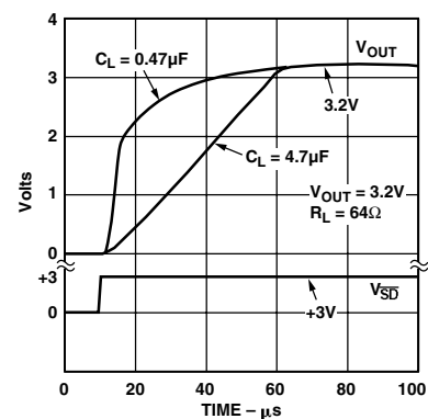
Figure 16. Turn On
