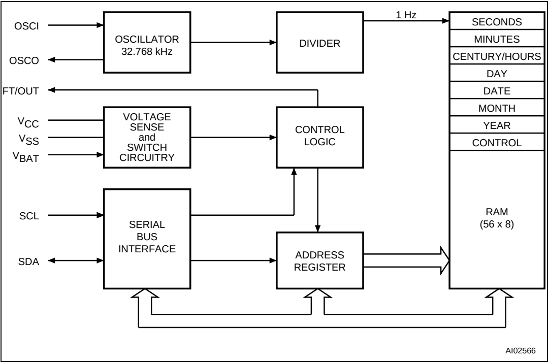
Figure 4. Block diagram
