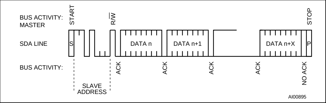
Figure 10. Alternative READ mode sequence
