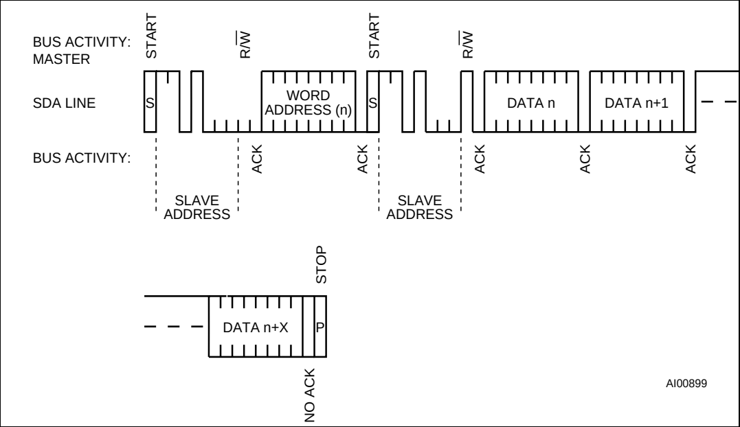
Figure 9. READ mode sequence
