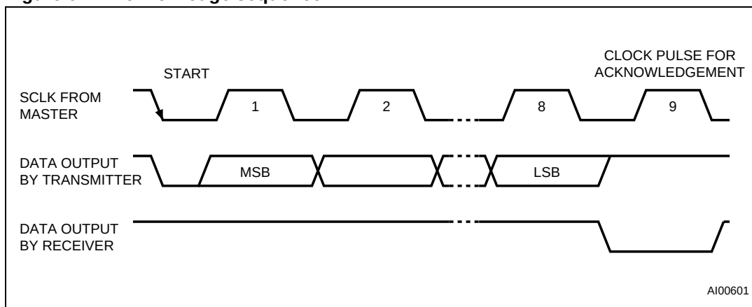
Figure 6. Acknowledge sequence
