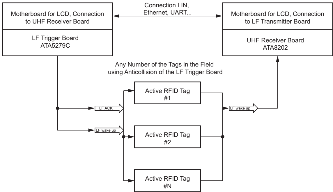
Figure 1-1. Atmel ATA6286-EK3 Development Kit System Diagram
