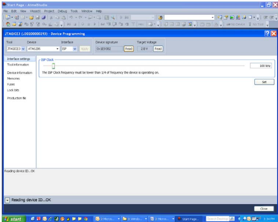
Figure 6-3. JTAGICE3 Interface Settings for RFID PCB
