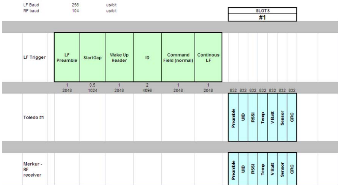
Figure 4-1. Typical Sequence in Normal Mode
