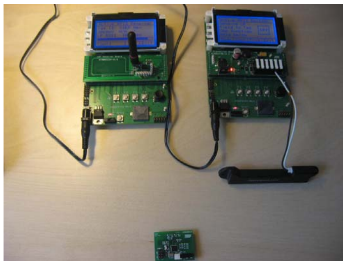
Figure 5-1. Operating Kit in Normal Mode
