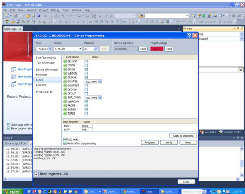
Figure 6-4. JTAGICE3 Fuse Settings for RFID PCB
