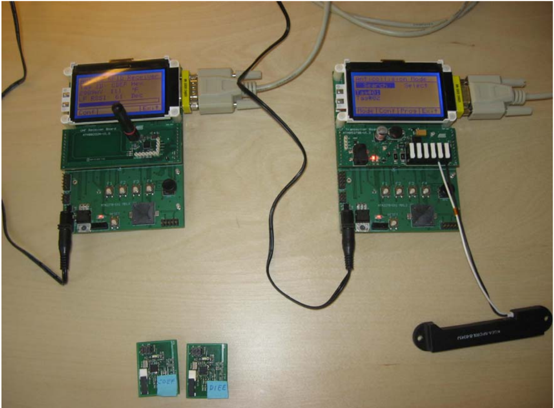
Figure 5-2. Operating Kit in Anticollision Mode
