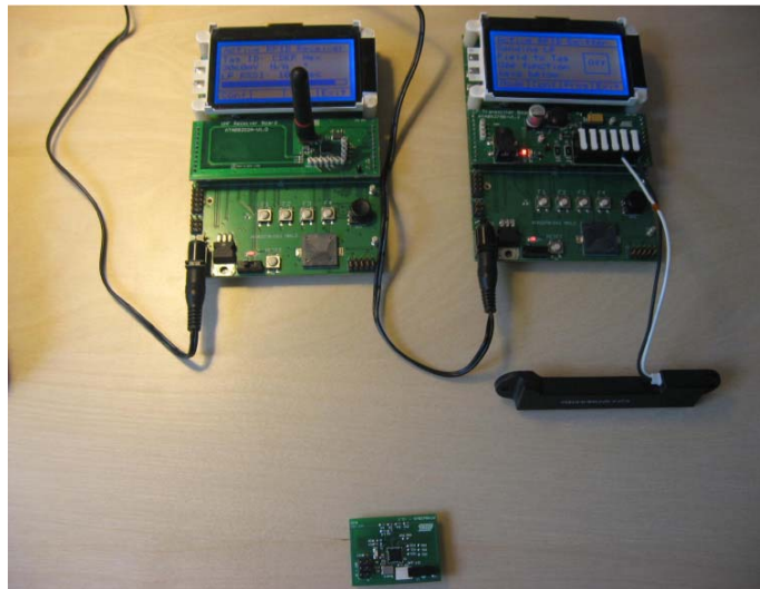
Figure 1-2. Atmel ATA6286-EK3 Development Kit
