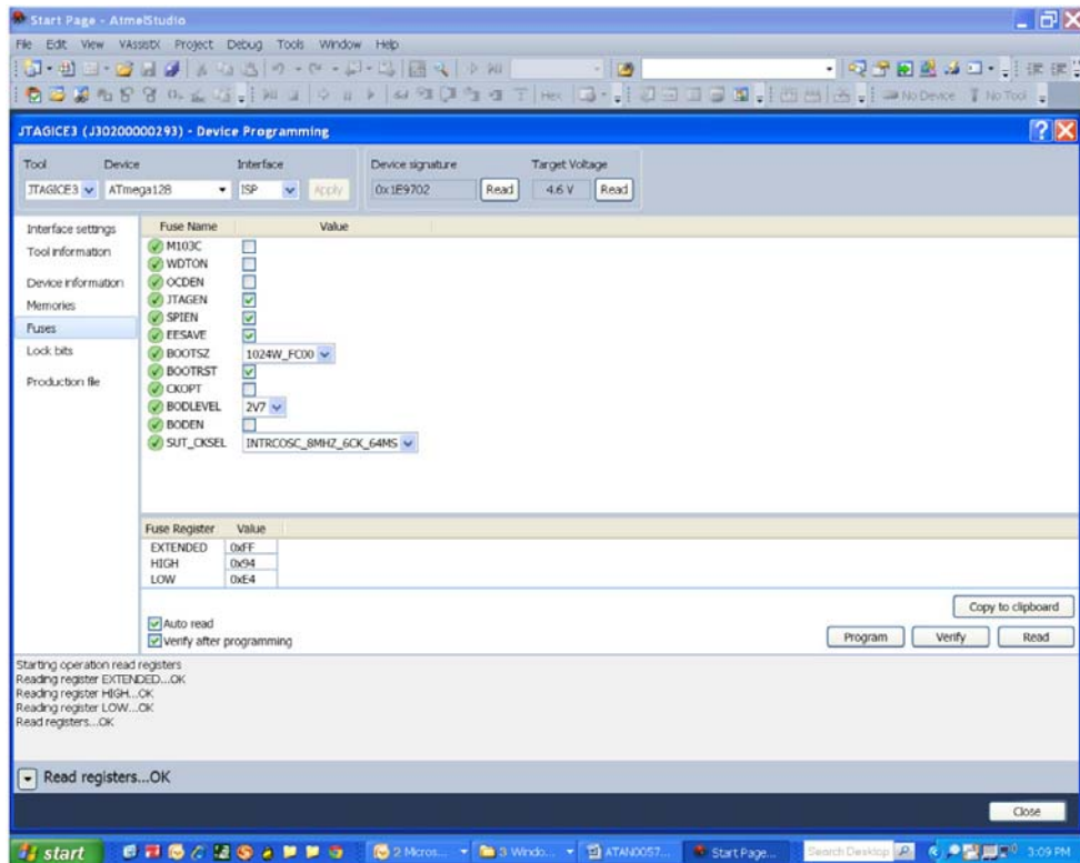
Figure 6-2. JTAGICE3 Fuse Settings for Mainboard
