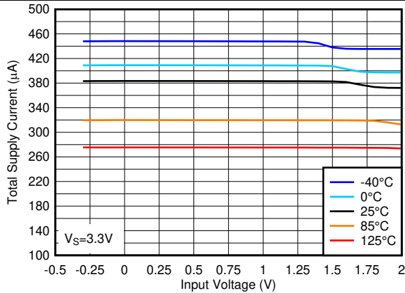
Figure 8. Total Supply Current vs. Input Voltage at 3.3V
