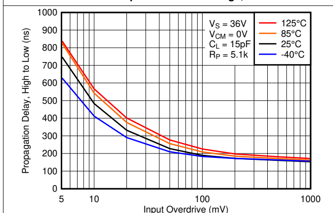
Figure 34. High to Low Propagation Delay vs. Input Overdrive Voltage, 36V
