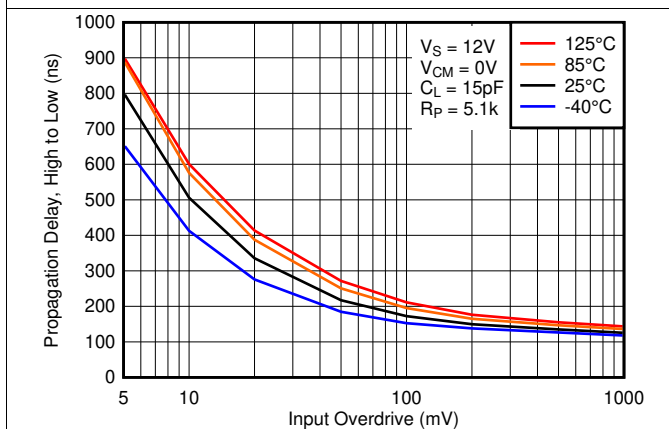
Figure 32. High to Low Propagation Delay vs. Input Overdrive Voltage, 12V
