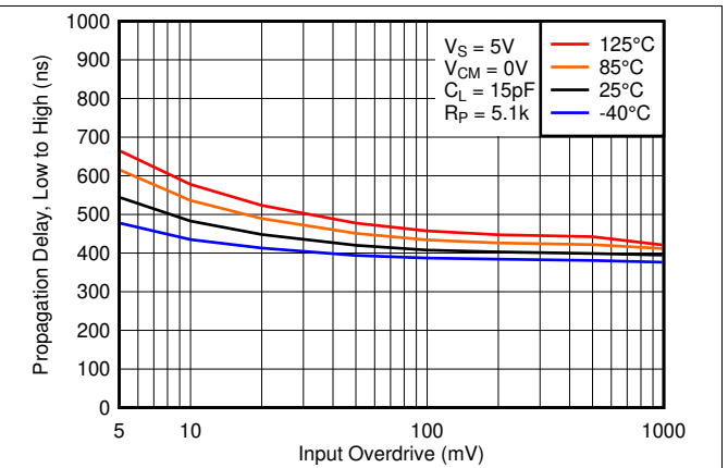
Figure 31. Low to High Propagation Delay vs. Input Overdrive Voltage, 5V
