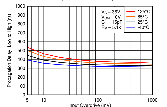
Figure 35. Low to High Propagation Delay vs. Input Overdrive Voltage, 36V
