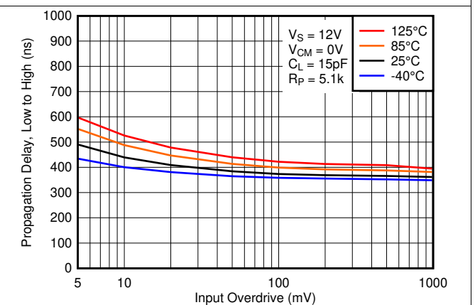
Figure 33. Low to High Propagation Delay vs. Input Overdrive Voltage, 12V
