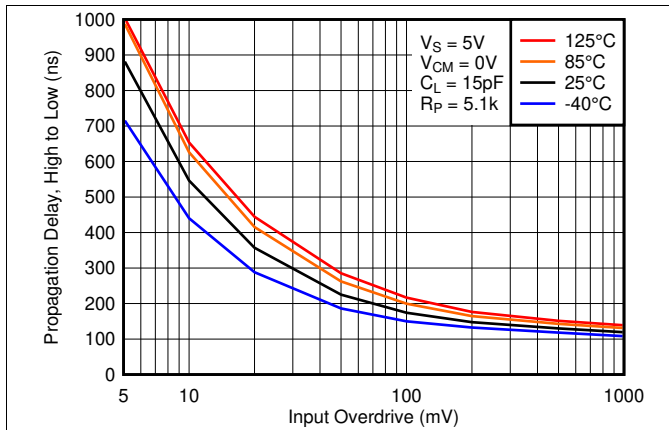
Figure 30. High to Low Propagation Delay vs. Input Overdrive Voltage, 5V
