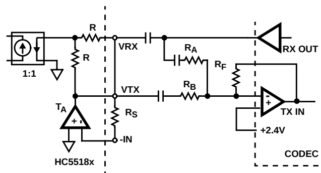
FIGURE 7. TRANSHYBRID BALANCE INTERFACE
